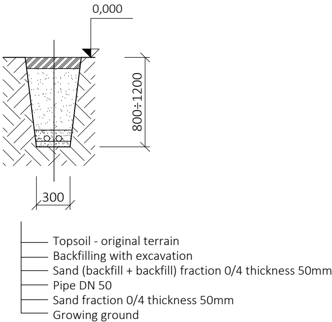
SAMPLE CROSS-SECTION OF THE PIPE INSTALLATION
