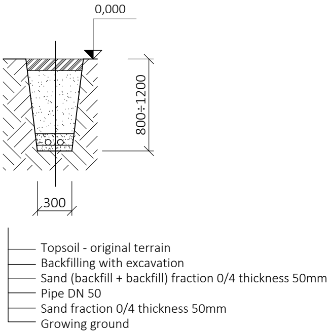
SAMPLE CROSS-SECTION OF THE PIPE INSTALLATION
